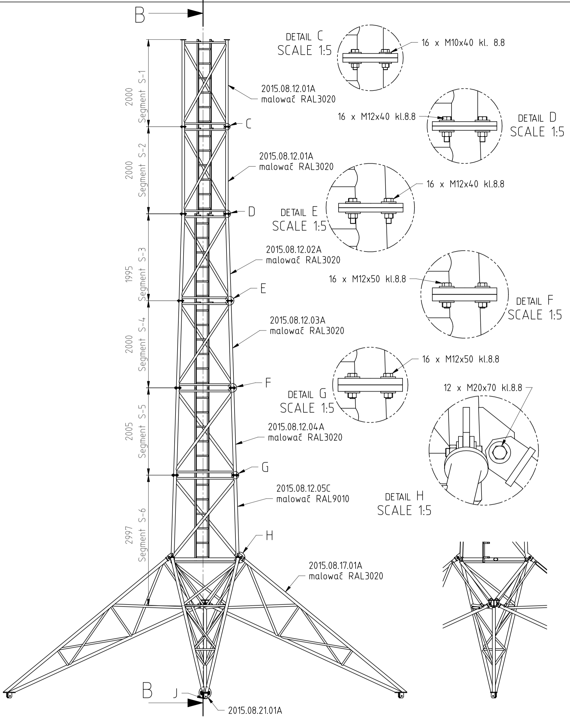
SECTION B-B
