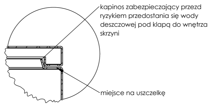
DETAIL B SCALE 1 : 5
